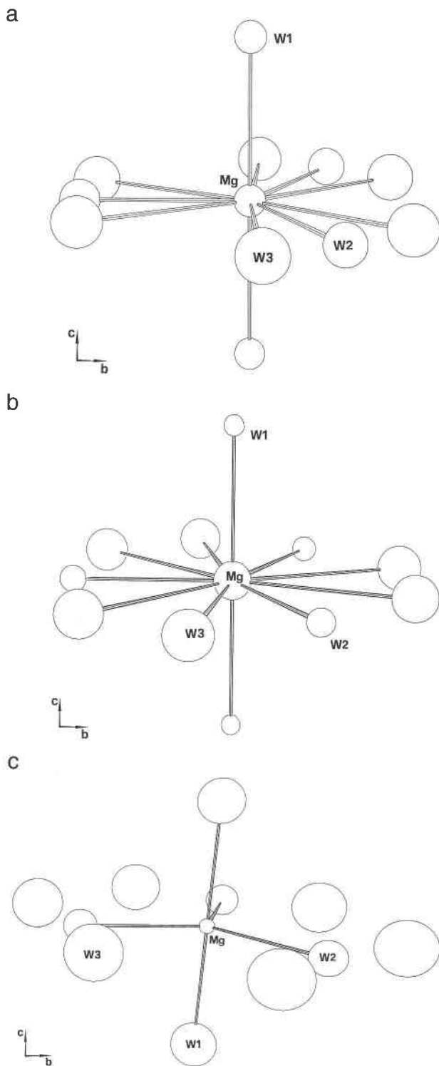
FIGURE 9. ORTEP plots of the Mg coordination environment in offretite. (a) offretite Mt. Semiol. Mg is bonded to two W1 at 1.96 Å, three W2 at 2.06 Å, and six W3 at 2.20 Å ( \text{W2}-\text{W3} = 0.98 Å; \text{W3}-\text{W3} = 1.96 Å) in an octahedral environment very similar to the one reported by Alberti et al. (1996); (b) Fittà1 W3 is at a greater distance ( \text{Mg}-\text{W3} = 2.40 Å) in an intermediate situation between the one described by Alberti et al. (1996) and the one proposed by Gard and Tait (1972) where Mg is bonded to two W1 (2 atoms per cell) at 2.00 Å, three W2 at 2.07 Å (2.4 atoms per cell), and six W3 (1.5 atoms per cell) at 2.40 Å ( \text{W2}-\text{W3} = 1.62 Å; \text{W3}-\text{W3} = 1.51 Å); (c) Fittà2 Mg coordination is close to the model proposed by Gard and Tait (1972), and Mg is bonded to two W1 (2 atoms per cell) at 2.07 Å, three W2 (2.8 atoms per cell) at 2.09 Å, and six W3 at 2.84 Å ( \text{W2}-\text{W3} = 1.58 Å). Mg is in a distorted fivefold coordination.
