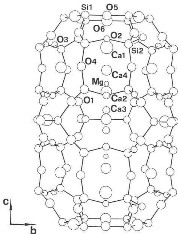
FIGURE 5. ORTEP plot of the erionite cage showing the positions of the extraframework cations. H 2 O molecules are not shown for the sake of clarity.
