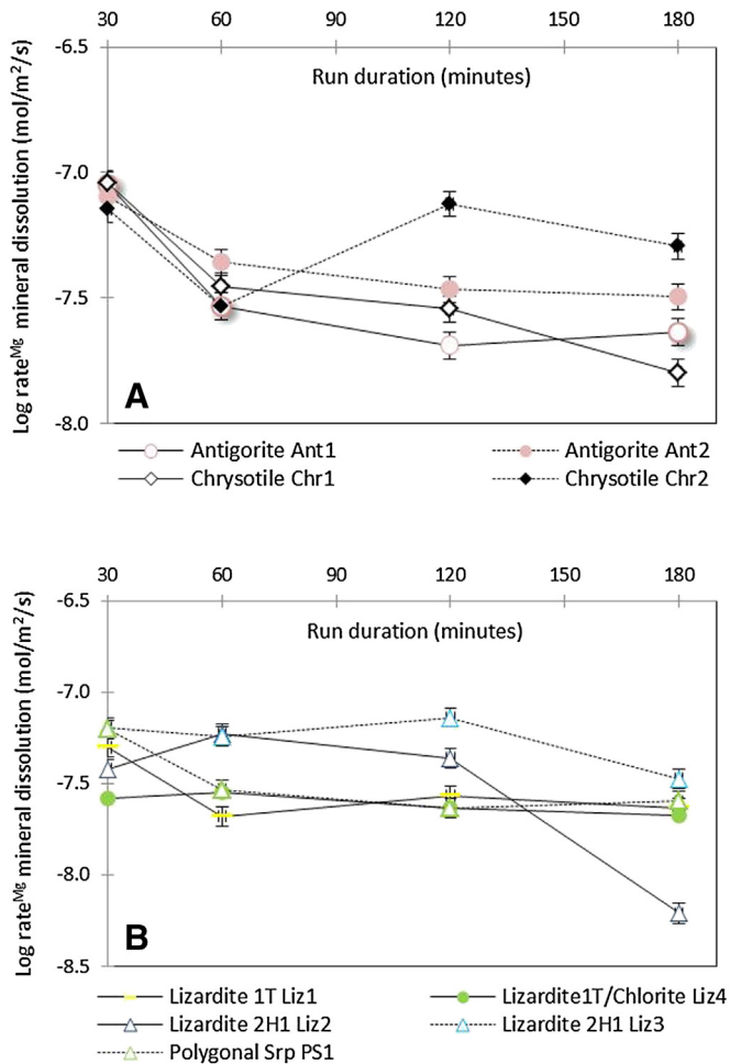
Fig. 5. The log rate ( \log R^{\text{Mg}} ) of mineral dissolution as a function of time: A) showing antigorite Ant1, Ant2, and chrysotile samples Chr1, Chr2; B) showing lizardite samples Liz1 1T , Liz2 2H1 , Liz3 2H1 , Liz4 1T and the polygonal serpentine sample PS1. The rates were calculated based on the concentrations of Mg in the leached solutions and normalised for changes in mineral stoichiometry. It is clear that lizardite 2H 1 and chrysotile exhibited higher values of \log R^{\text{Mg}} than antigorite and Liz1 1T , PS1; largely corresponding to the degree of mineral dissolution illustrated by the \text{Mg}^{\text{EE}} .
