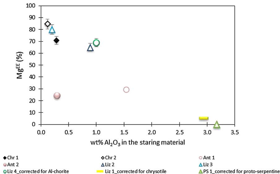
Fig. 11. Mg EE as a function of Al 2 O 3 content in the starting material. Three samples were plotted after appropriate correction, i.e. Liz1 1T _corrected from chrysotile; Liz4 1T _corrected for Al-chlorite and PS1_corrected for proto-serpentine. An inversely proportional relationship between the Al 2 O 3 content and Mg EE is apparent for all, but antigorite samples.
