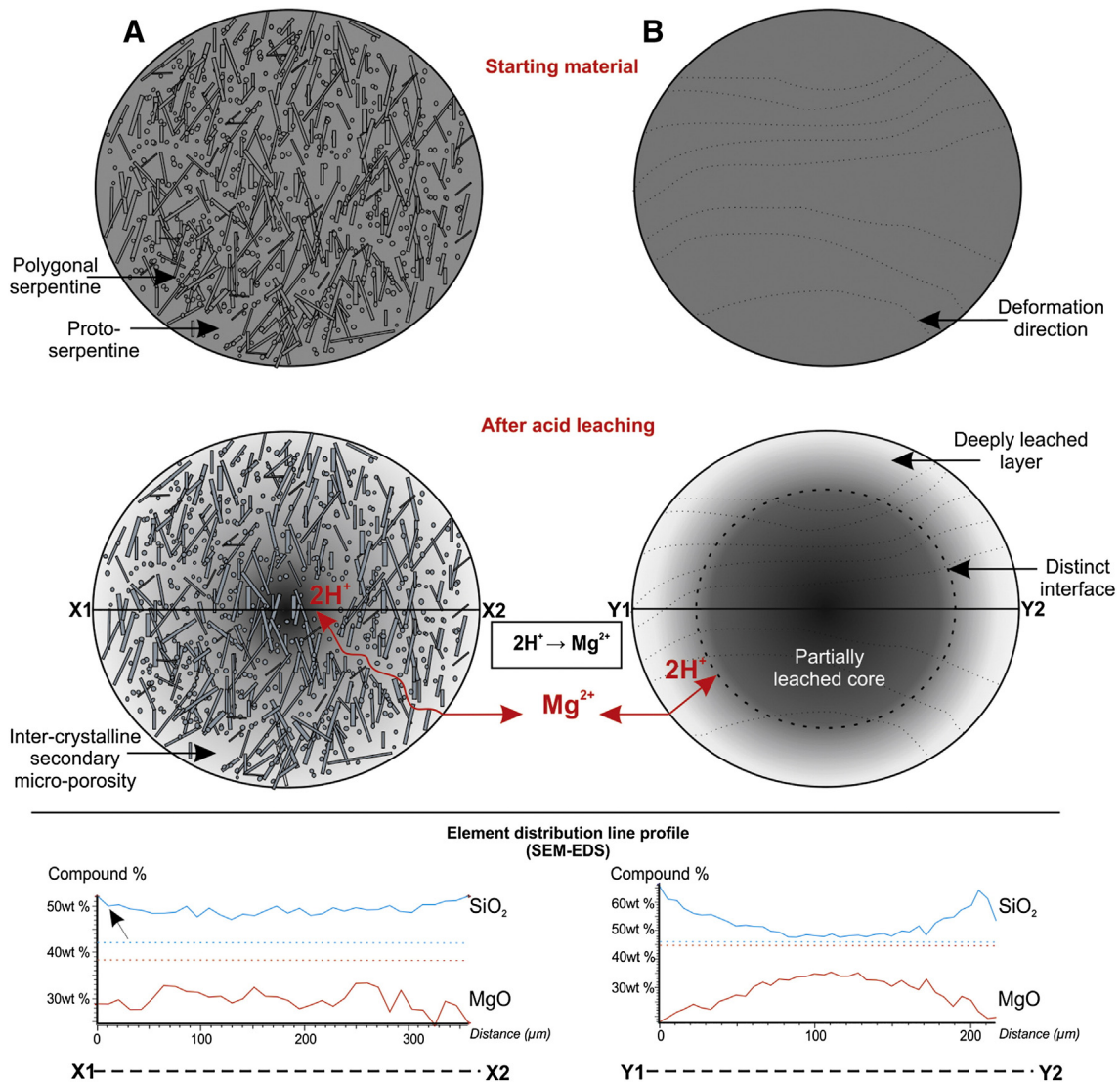
Fig. 10. Schematic representation of a conceptual model for siliceous layer formation through 2\text{H}^+ \rightarrow \text{Mg}^{2+} exchange in two types of lizardite-rich particles ( \approx 400 \mu\text{m} across), A) before and after leaching particle with elongate crystals of polygonal serpentine set in proto-serpentine matrix, collectively representing a dual micro-texture and B) before and after, distinctively deformed but texturally homogeneous particle of generally poorly-crystalline lizardite 2\text{H}_1 (Liz3). The associated measured (EDS) element distribution line profiles show roughly uniform chemical gradient in PS1 (with the fluctuation corresponding to the compositional duality of the sample) and sharper gradient between the siliceous layer and the core of the particles in Liz3. The faint straight lines on the element distribution profiles represent the oxide composition of the starting material, blue for \text{SiO}_2 and red for \text{MgO} . (For interpretation of the references to color in this figure legend, the reader is referred to the web version of this article.)
