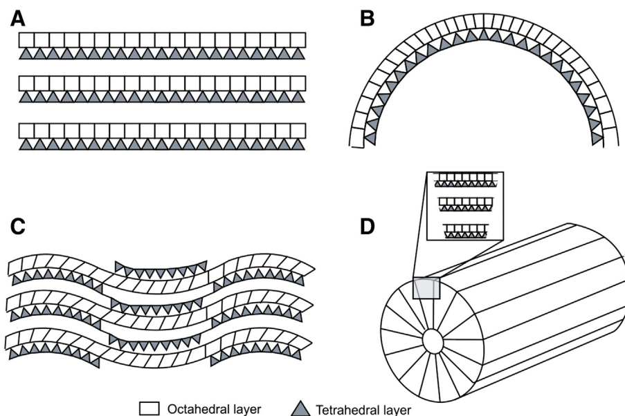
Fig. 1. Schematic representation of serpentine minerals crystal structure, including: A) flat layer lizardite, B) tubular chrysotile, C) modulated antigorite (Mevel, 2003) and D) polygonal serpentine [adapted from (Cressey et al., 2010)].
