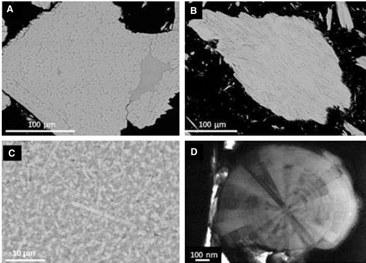
Fig. 3. Backscattered (A–C) and transmission electron images showing: A) texturally heterogeneous lizardite-dominated particle (Liz1) with lizardite 1T intergrown interstitially with chrysotile (lower BSE contrast); B) texturally homogeneous antigorite (Ant2) with tightly intergrown and aligned crystals; C) dual texture of short-fibre polygonal serpentine and a proto-serpentine matrix (lower BSE contrast) (PS1), D) Cross-axis HRTEM image of polygonal serpentine fibre (PS1). Image D, courtesy of M Fay and C Parmenter (Nottingham Nanotechnology and Nanoscience Centre).
