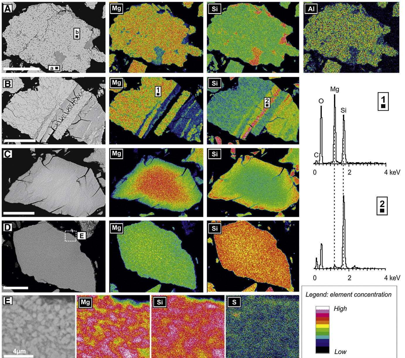
Fig. 7. Backscattered electron images of representative acid-leached particles of serpentine minerals (180 min solid residuum), and associated X-ray element distribution maps, showing: A) Liz1 1T with preferentially leached serpentine, tentatively assigned to chrysotile ( a ) and intact aluminous-lizardite ( b ); B) Liz2 2H1 with deeply Mg-leached zones, now siliceous residuum as illustrated in the EDS X-ray spectrum 2; C) Liz3 2H1 with leached micro-scale layer texture with deeply Mg-leached reaction rim and partially altered particles core. Note the sharp contact between the leached and partially leached zones; D) PS1 with subtly Mg-leached rim, and generally a roughly uniform transformation; E) high magnification of particle “D”, showing a dual nature of this sample with polygonal serpentine, represented by bright BSE laths in a matrix of proto-serpentine. The associated maps clearly indicate that the matrix is Mg-depleted and Si-enriched, proving that its leaching contributed most to the Mg EE as plotted in Fig. 4. The scale bar, unless specified, corresponds to 100 μm, showing that all the particles are roughly the same size.
