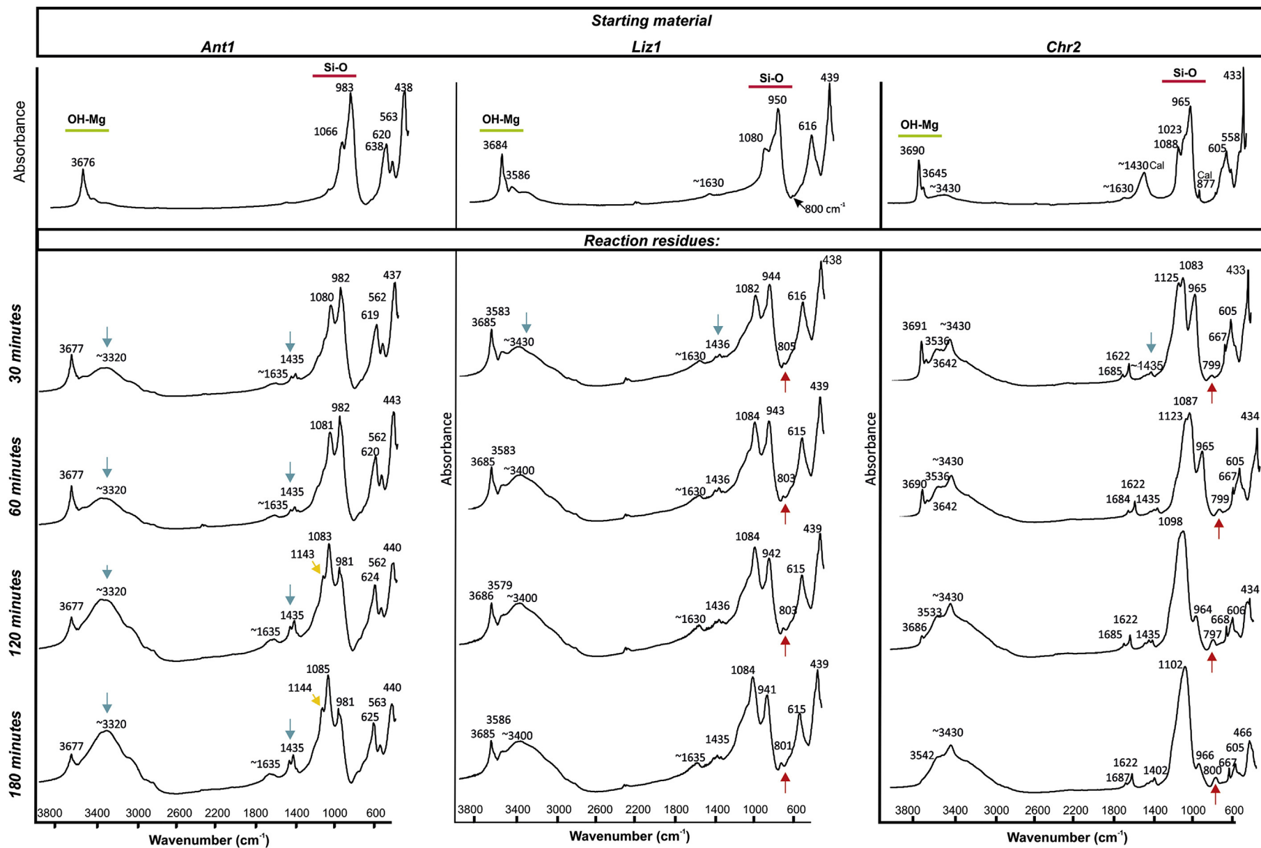
Fig. 9. FTIR spectra of (a) Ant1 (b) Liz1 1T and (c) Chr2 and associated reaction residues; reflecting the time dependent structural modifications that occurred during acid leaching. The blue arrows correspond to secondary bousingaultite, the yellow arrows indicate a low intensity peak attributable to quartz, and the orange arrows indicate a peak corresponding to amorphous silica. (For interpretation of the references to color in this figure legend, the reader is referred to the web version of this article.)
