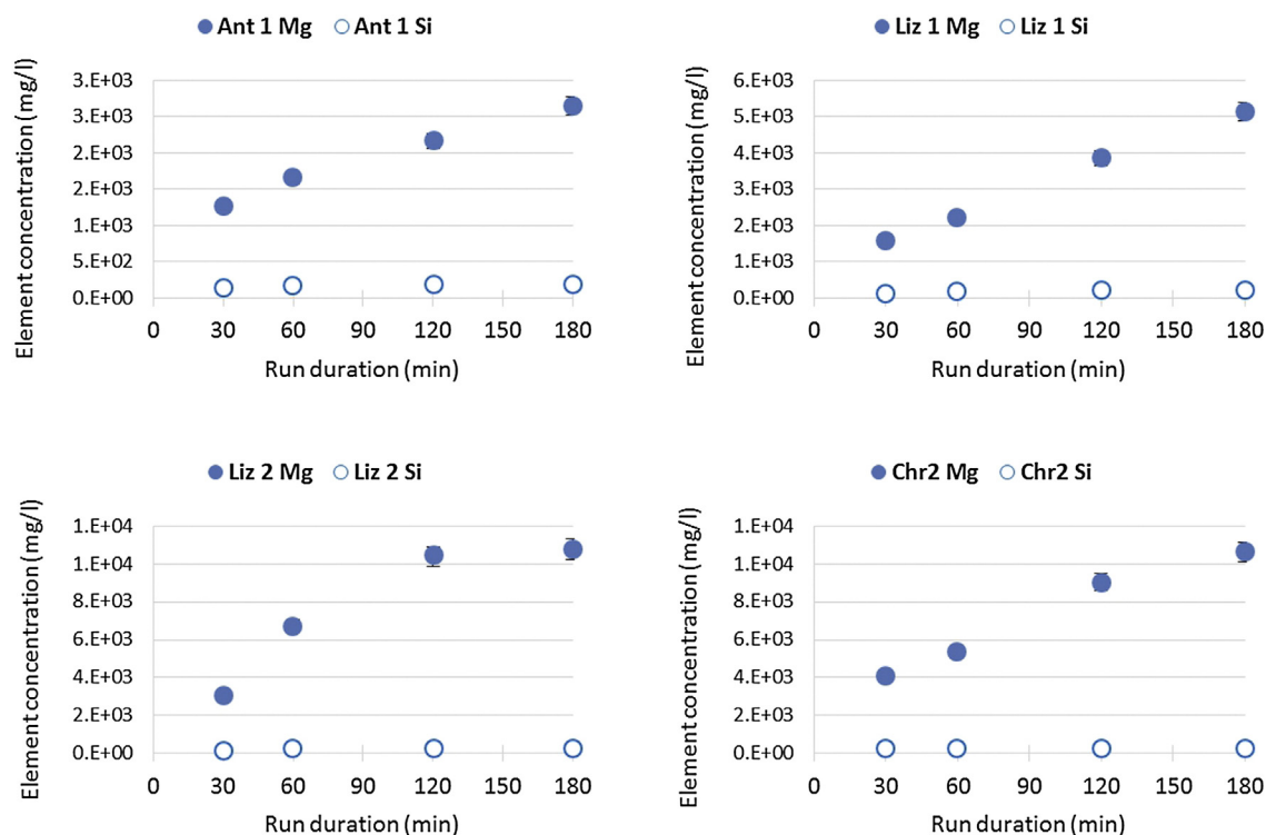
Fig. 6. Time evolution of Mg and Si concentration in the leachates of Ant1, Liz1 1T , Liz2 2H1 and Chr2; all plots clearly indicate an incongruent release of the two cations into the solution.
