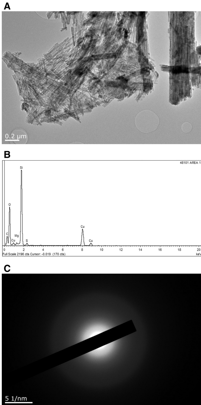
Fig. 8. TEM image of a bundle of acid-leached chrysotile (180 min Chr2) (A) fibres and corresponding EDS (B) spectrum and SAED pattern, (C) indicating that the leaching residuum is silica-dominated and amorphous. Trace amounts of Mg and S were also detected, originating from the mineral and solution, respectively; whilst the prominent Cu and C peaks in the EDS spectrum are from Cu grid and C-based film, holding the sample.
