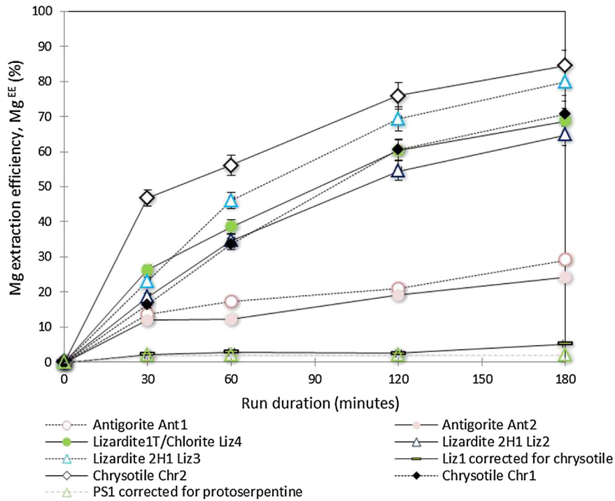
Fig. 4. Mg EE (%) from structurally different serpentine minerals, showing high efficiency of chrysotile, Al-poor and two-layer polytype of lizardite and low efficiency for antigorite, Al-lizardite 1T and Al-polygonal serpentine. It is noted that the data points for PS1 are tentative only (hence faint line), due to uncertainty related to proto-serpentine content. The graph was prepared based on XRF data obtained from starting materials and four solid reaction residues. The error bars show possible 5% variation.
