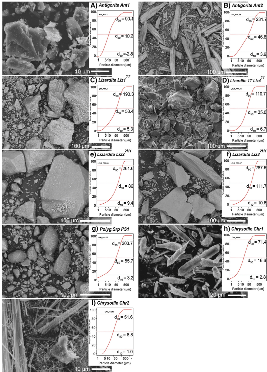
Fig. 2. Secondary and backscattered electron images illustrating the diversity of particle sizes and shapes of the milled starting material. Corresponding particle size distribution curves are plotted as a function of % cumulative volume.
