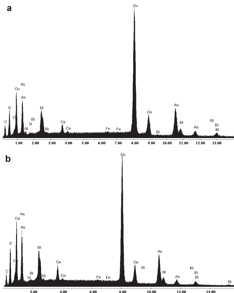
Fig. 1. EDX analyses of (a) the Majuba mixite and (b) the Boss mixite.
