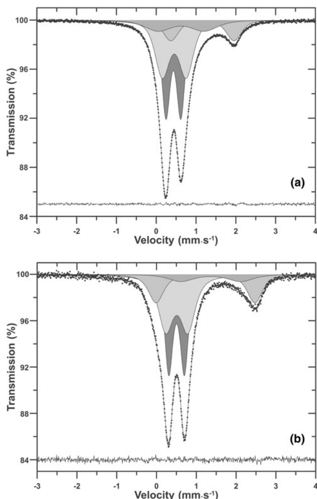
Figure 5. Mössbauer spectra of a mixture of dmitryvarlamovite, a \text{Fe}^{3+}\text{NbO}_4 phase and columbite-(Fe) at (a) room (295 K) temperature and (b) 90 K.
