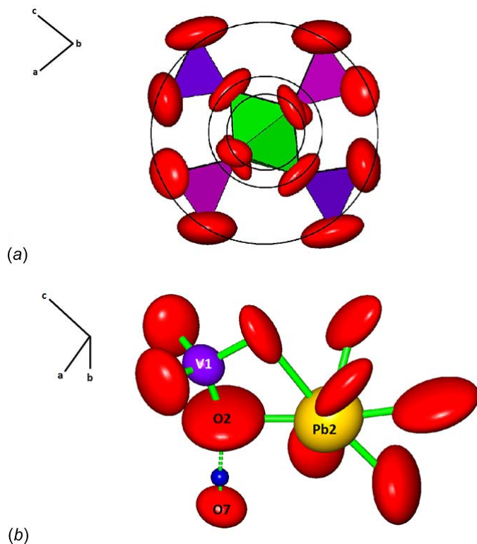
Figure 3 ( a ) View of the \infty^1[Mn^{3+}(VO_4)_2OH] chain looking down [010]. The black rings represent different radii that correlate with the progressive increase of the libration component of oxygen atoms further away from the centre of the chain. Purple and violet tetrahedra and green octahedra represent V1O_4 , V2O_4 and [MnO_6] , respectively. Red ellipsoids represent O atoms; ( b ) large O2 disk-shaped ellipsoid oriented perpendicular to the V1-O bond (anisotropic displacement ellipsoids at the 99% probability level). Note the hydrogen bond O2\cdots H-O7 (dashed lines). Purple, yellow and red ellipsoids represent V1O_4 , [Pb_2O_8] and O atoms, respectively. The blue sphere represents the H atom.
