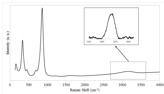
Figure 4 Raman spectrum of brackebuschite. The weak Raman band around 3145 cm^{-1} is assigned to the OH stretching vibrations associated with the OH group ( \nu_{OH} ).
